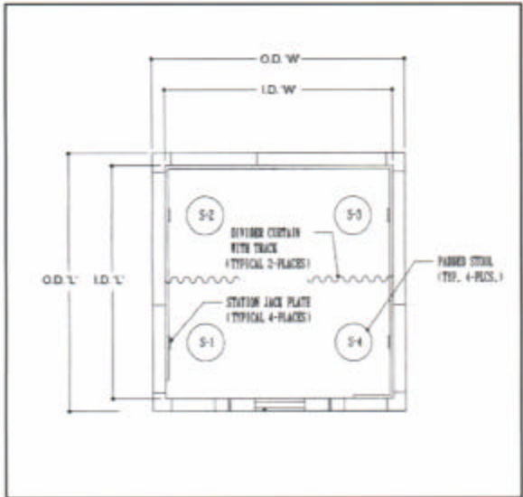
40m Series Plan
