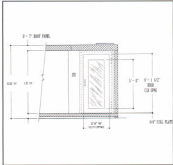
40m Series Typical Elevation
