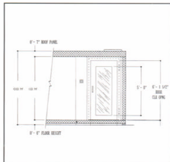
120m Series Typical Elevation
