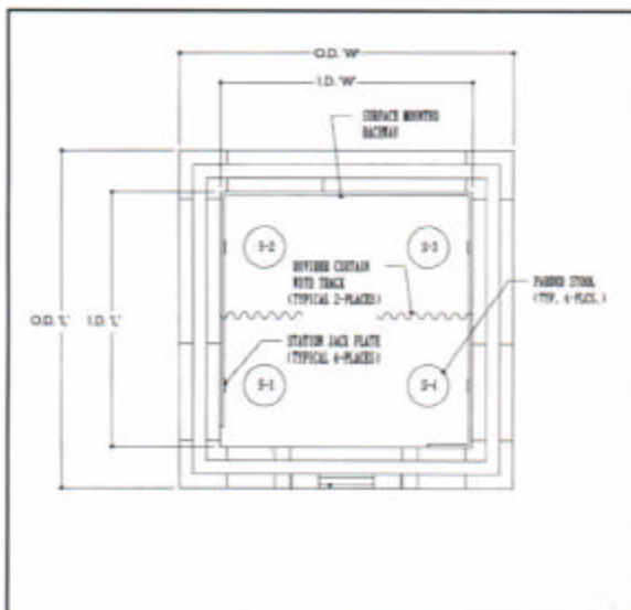
120m Series Plan
